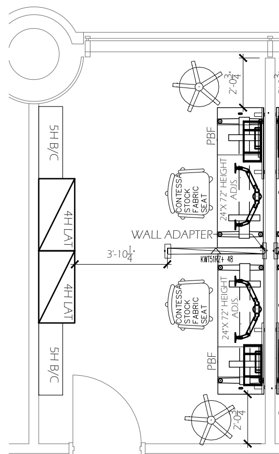
1 DOUBLE OFFICE COLUMN TYPICAL 1 FURNITURE PLAN SCALE: N.T.S.
