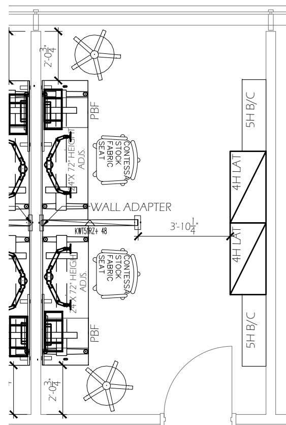
1 DOUBLE OFFICE TYPICAL 2 FURNITURE PLAN SCALE: N.T.S.
