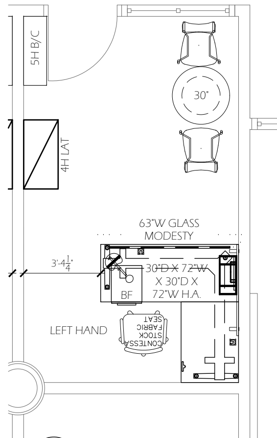
1 LEFT HAND TYPICAL 4 FURNITURE PLAN SCALE: N.T.S.
